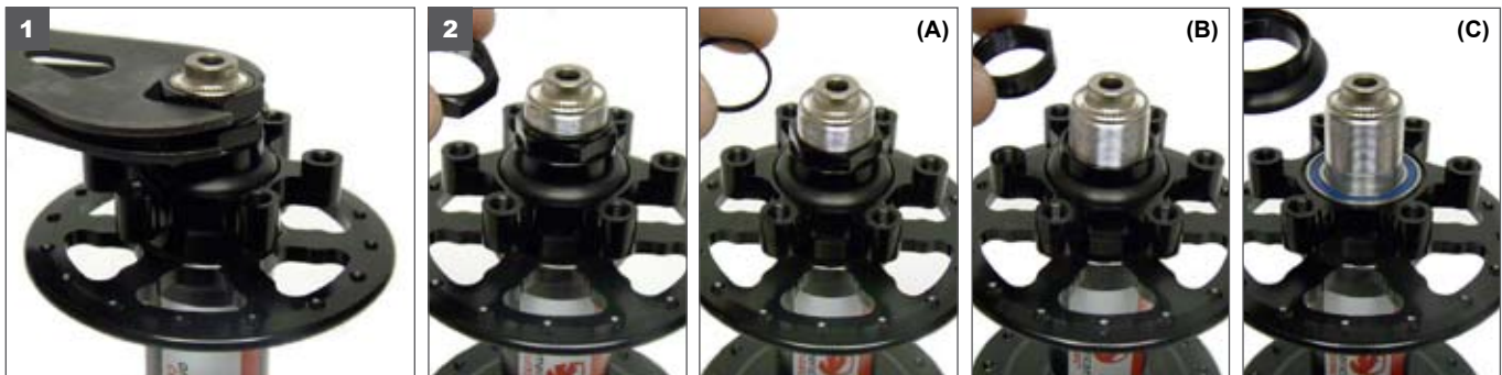
1. Using two 19mm cone wrenches, loosen the lock and adjusting nut. 2. Remove lock nut. A. Some hubs have a 1.5mm axle spacer. B. Remove adjuster nut. C. Remove spacer with attached dust seal.
