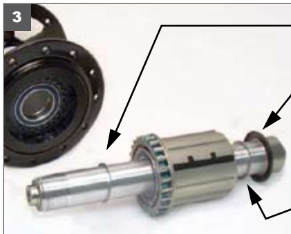
3. Separate cassette body and axle from the hub shell by grabbing the body and pulling out from the drive side. 4. Remove large black pawl seal.
