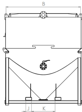
FRONT
