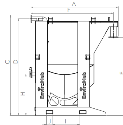
RIGHT
