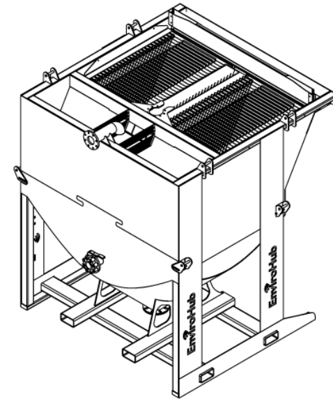
ISOMETRIC
