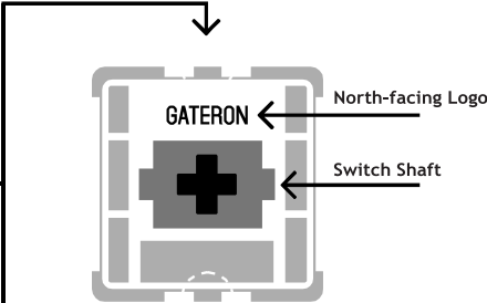
The Switch Puller tool aligns Vertically to the Switch to unclip the plastic securing the switch to the plate.
