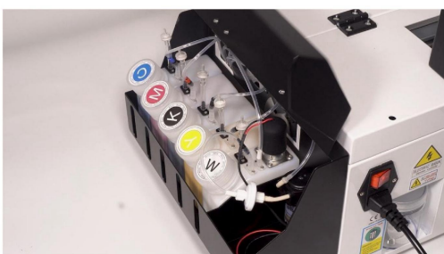
Step 35. Recognize the colors. C refers to cyan ink, M refers to magenta ink, Y refers to yellow ink, K refers to black ink and W refers to white ink
