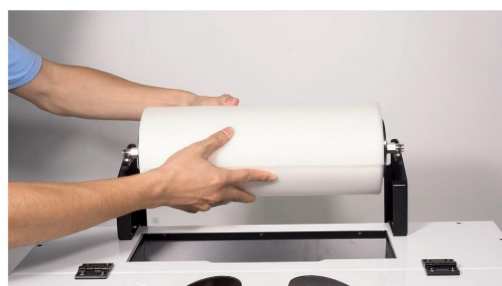
Step 18. Put the film roll onto the bracket. (The printable side with coating facing up)
