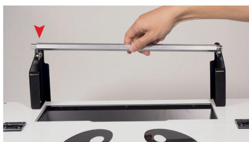
Step 7. Put the roller bar onto the brackets.
