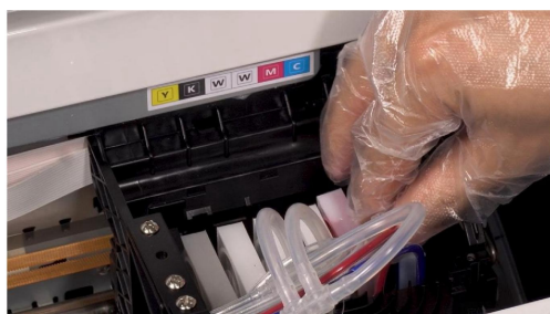
Step 39. Put the cartridge back in place after extracting.
