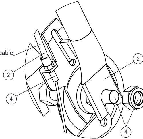
STEP 2: Attach wheel to front part
