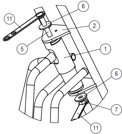
STEP 1: Attach front part to rear part
