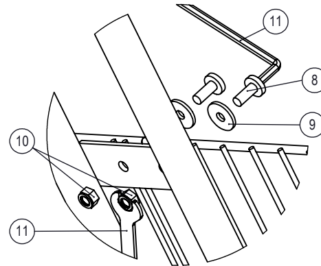
STEP 4: Attach basket to front part
