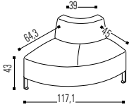
F55 Non Symetric Curved Module Left With Backrest
