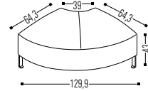
F43 Curved Symetric Module 64 cm Side
