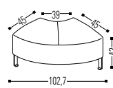
F42 Curved Symetric Module 45 cm Side
