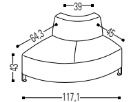
F35 Non Symetric Curved Module Left With Backrest
