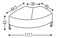
F45 Non Symetric Curved Module Left
