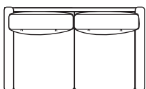
76" Sofa 76" w x 38" d x 34" h
