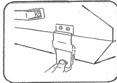
Loosen securing latches at the back of the Stealth NB (It is very important to make sure that the front securing latches have been released before lifting or the hinge mechanism may get bent in the process).
