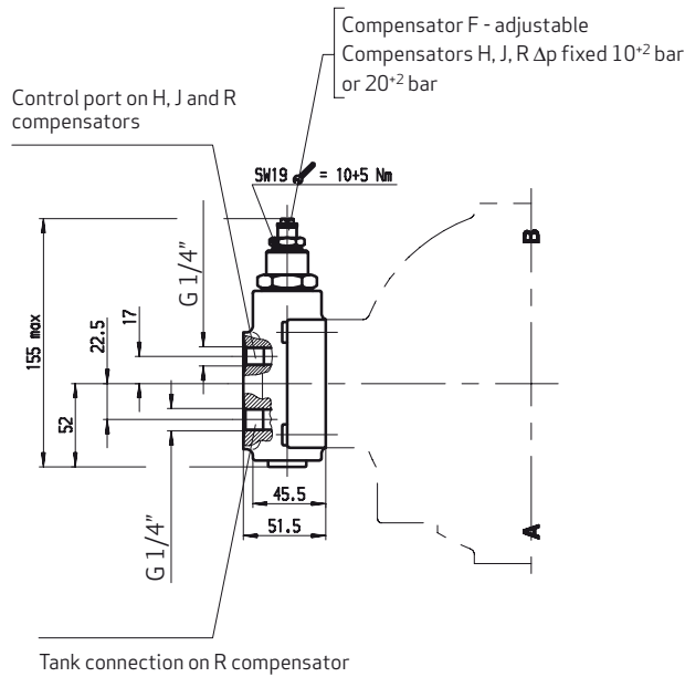
RKP 19/32/45
