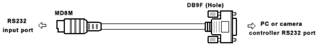
Figure1-6 RS-232 Diagram
