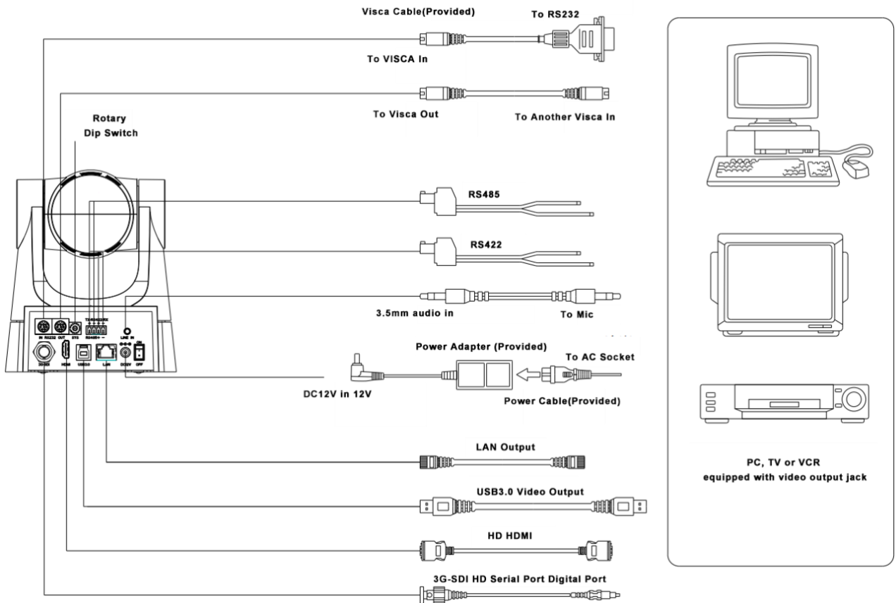
Figure1-5 Interface Diagram
