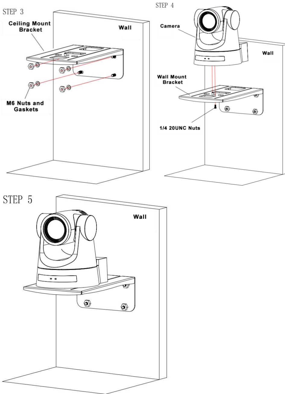
Figure1-2 Steps of Wall Mount
