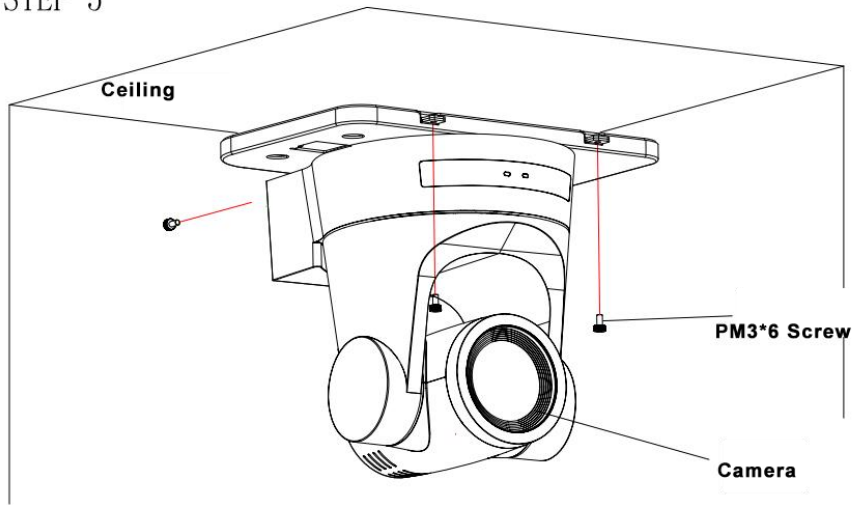
Figure1-3 Steps of Ceiling Mount
