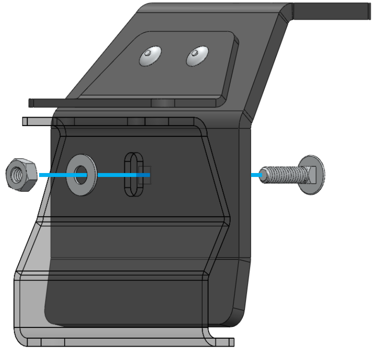
1. HORIZONTAL HARDWARE SET
