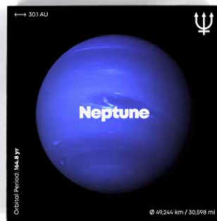
Neptune
