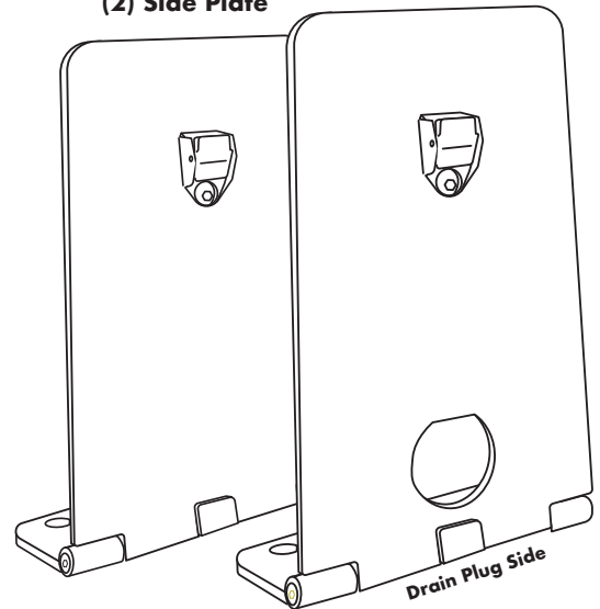
(2) Side Plate
