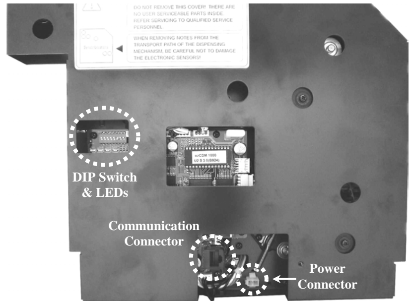
LG Dispenser (side view)
