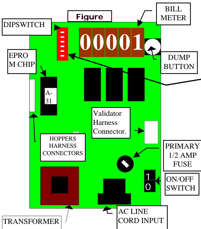
FIGURE 2 (THIS IS NOT THE DipSwitch BANK FOR SETTING THE BILL DENOMINATIONS. (For those dip switches go to page 10.)
