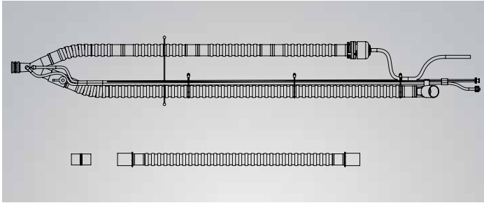
15090-101 Patient circuit w/PEEP, 22 mm SPU single heated wire, Fisher & Paykel (10/pkg)
