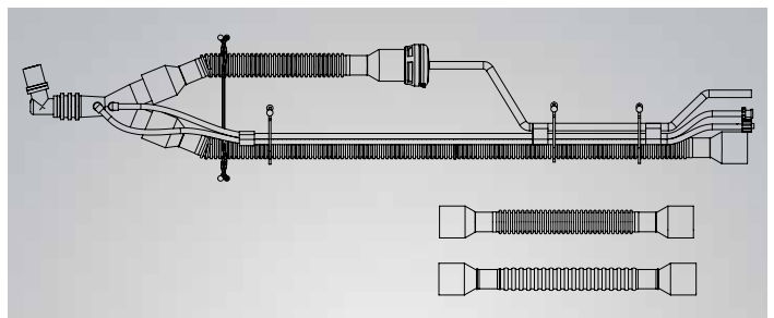
14859-001 Patient circuit w/o PEEP w/elbow, 15 mm SPU (10/pkg) 1.8 m x 15 mm insp limb, wye, elbow and 61 cm x 15 mm exp limb
