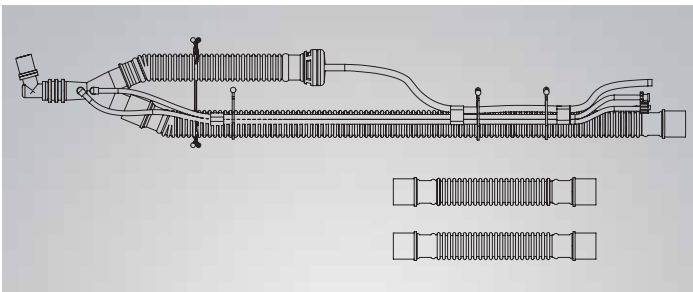
14858-001 Patient circuit w/o PEEP w/elbow, 22 mm SPU (10/pkg) 1.8 m x 22 mm insp limb, wye, elbow and 61 cm x 22 mm exp limb
