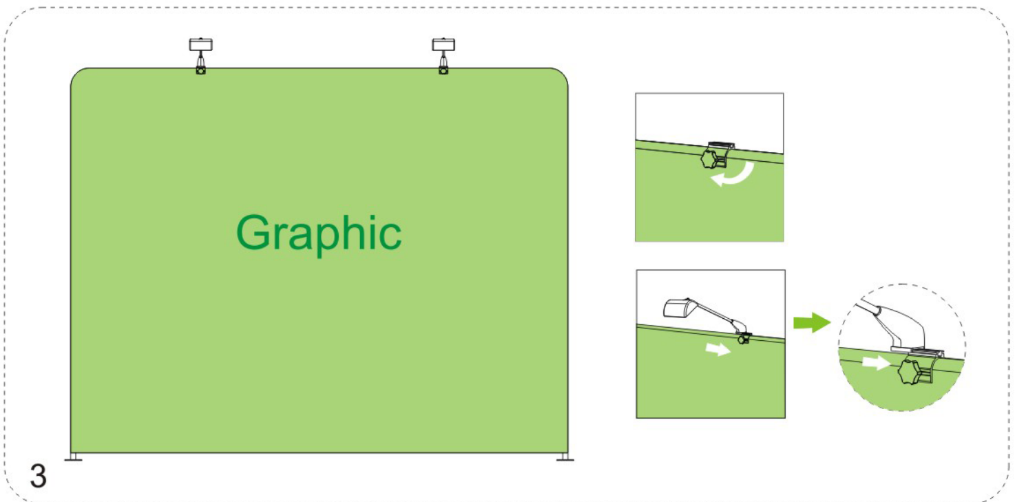
3 Put the light clip on the top of display and fix it with screw, then connect the light and the clip
