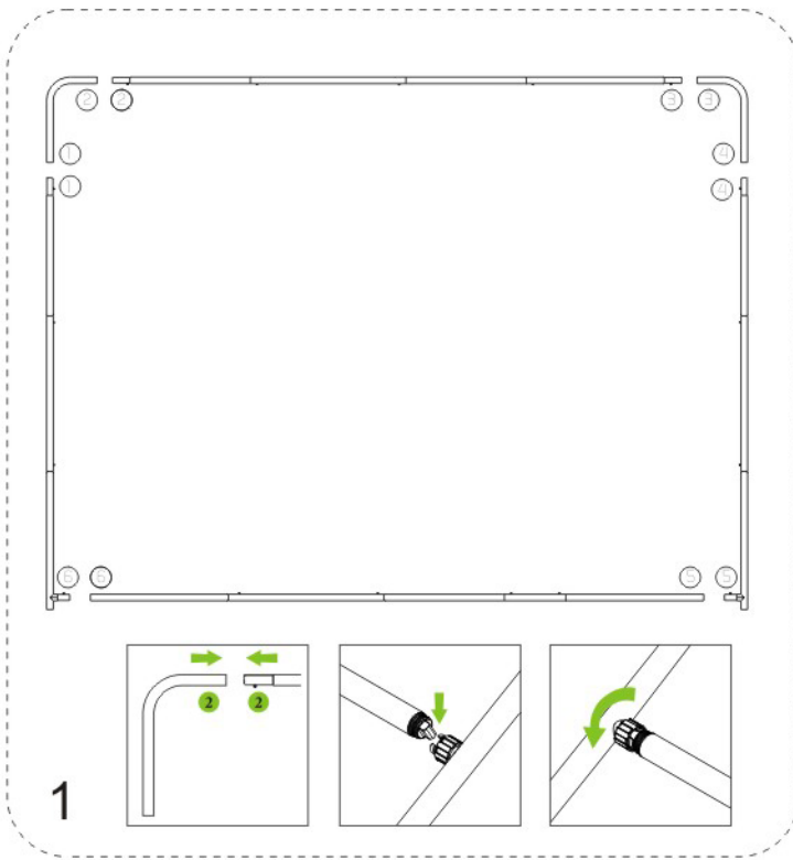
1 Connect tubes of the frame (there are number labels on tubes)
