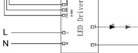
Wiring diagram
