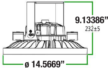
Surface Mounted with Motion Sensor
