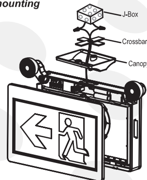
Ceiling mounting
