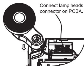
Lamp head (forward)
