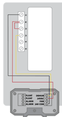
4041649 HONEYWELL HUMIDIPRO WIRING DIAGRAM
