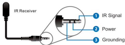
IR RECEIVER
