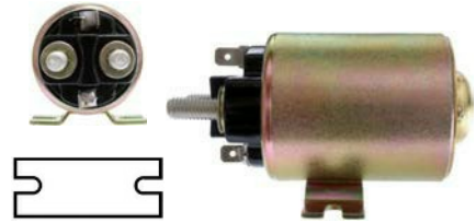
333153 Solenoid Manufacturer: Bosch r eplacing: 19024761 12 V, 150 a, Intermittent load 800 Amp., OD 51.75, Coil bolt M8, seconds 5, No./ terminals 4 Silver contact. Insulated return. alternative no.: 131373, 131373Z
