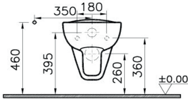
Standart baglanti Standard connection Standard Verbindung
