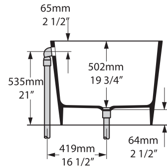
Section BB Shown with K17 waste kit
