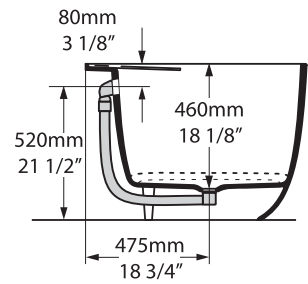
Section BB Shown with K60/K61 waste kit
