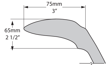
Rim Detail
