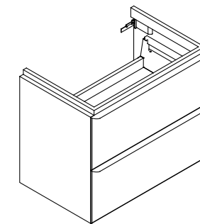
4.1016.2 X. 635 mm Y. 520 mm Z. 410 mm
