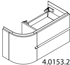
4.0153.2 X. 840 mm Y. 450mm Z. 375mm
