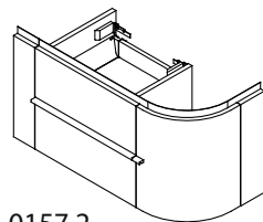
4.0157.2 X. 760 / 830mm Y. 450mm Z. 375mm
