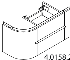
4.0158.2 X. 760 / 830mm Y. 450mm Z. 375mm
