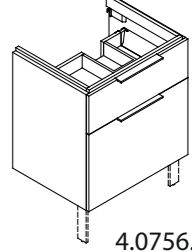
4.0756.2 X. 595 mm Y. 615 mm Z. 455 mm
