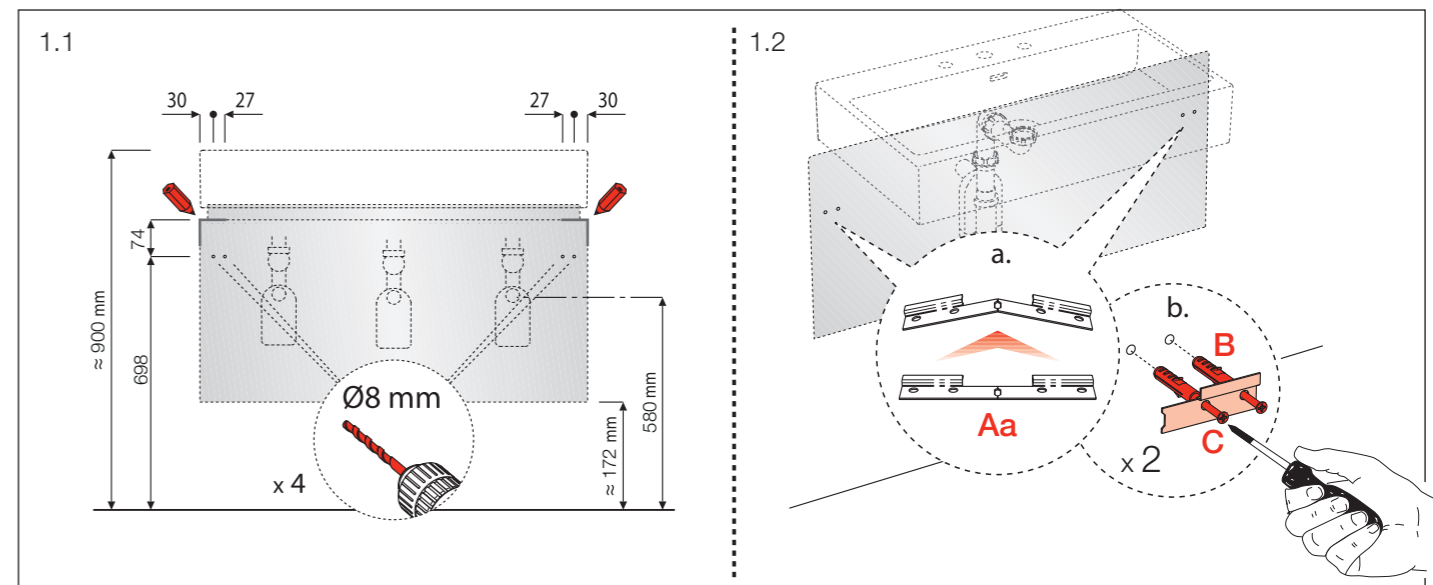
4.0760.1 X. 895 mm Y. 615 mm Z. 455 mm
