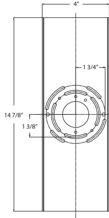
BACK PLATE DIMENSIONS
