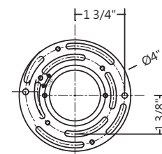
Mounting Ring Dimensions
