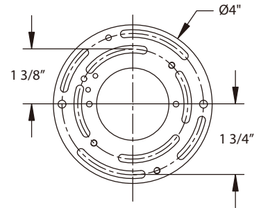
Mounting Plate Dimensions
