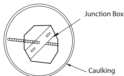
Fig.3 Sealing
