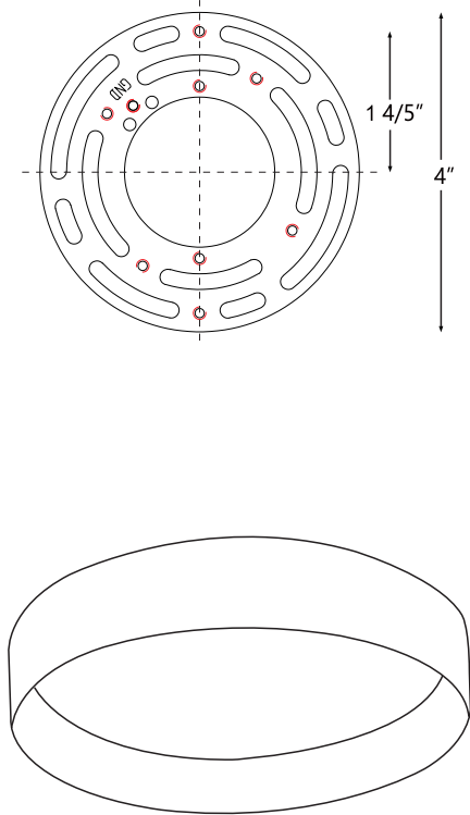
Back Plate Dimensions
