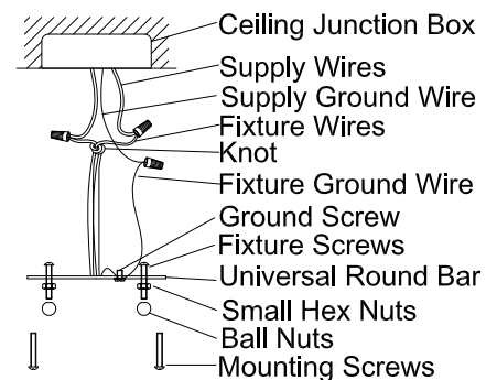
Wiring Drawing (2)
