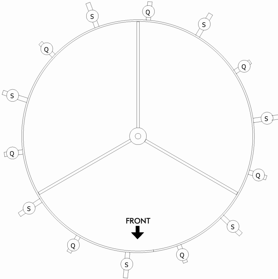
TOP VIEW TIER 1
