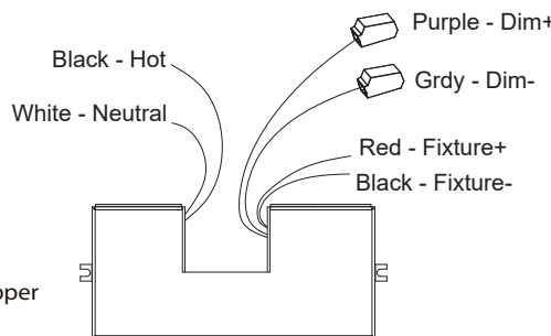
Fig. 3 Driver Wires
