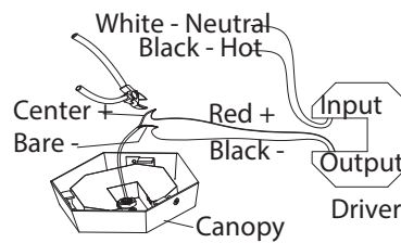
Fig.3 Driver Wires
