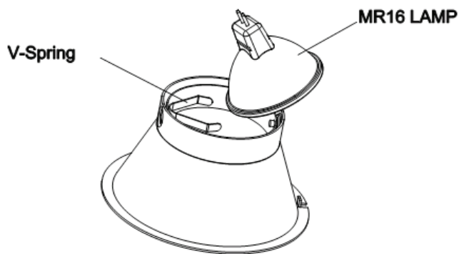
Detailed view: lamp insertion
