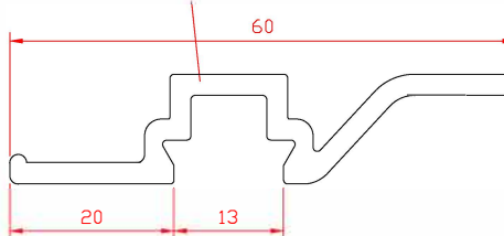
PSV/37/870 PILLAR TRIM - 60mm WIDE
