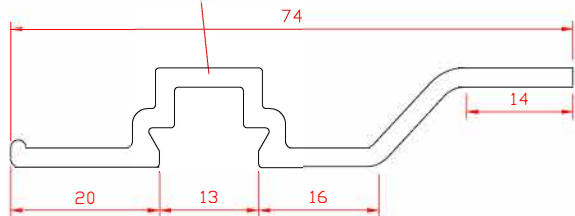
PSV/61/285 PILLAR TRIM - 74mm WIDE
