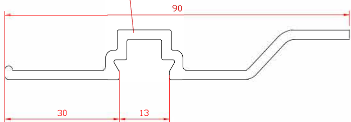
PSV/37/872 PILLAR TRIM - 90mm WIDE
