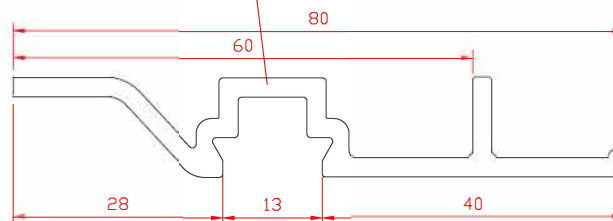
PSV/61/286 PILLAR TRIM - 80mm WIDE
