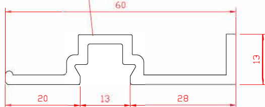
PSV/37/871 PILLAR TRIM - 60mm WIDE
