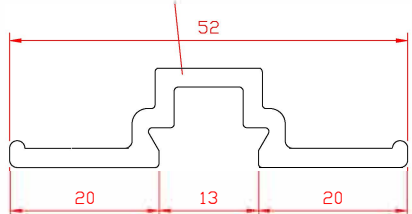
PSV/99/389 PILLAR TRIM - 52mm WIDE
