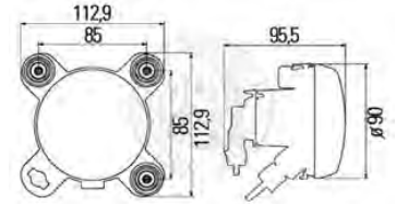
H1 Main Beam Headlamp
