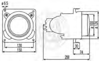
H1 Headlamp
