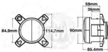
H11 Main Beam Headlamp
