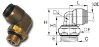
90° Elbow, Male Metric Thread
