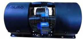
Pedro Sanz Brushless Blower Frontbox Caetano / Sunsundegui, 24V
