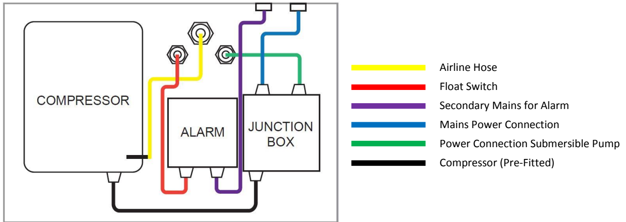
Figure 14: Connections inside External Air Blower Housing (Pumped Outlet Version)
