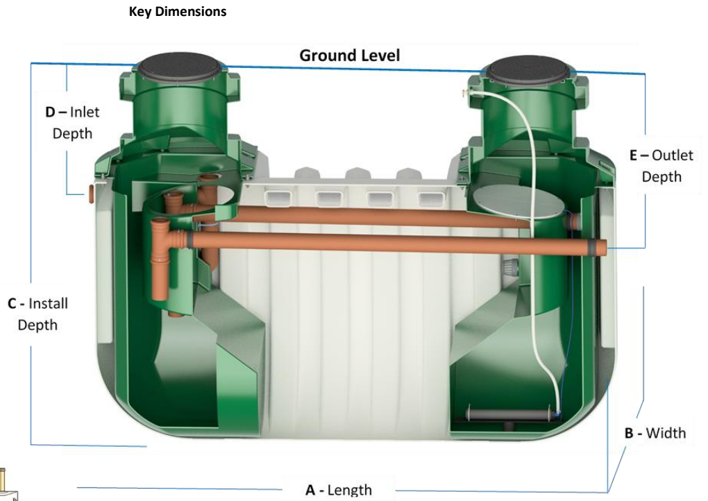
Figure 3: HydroClear 12 Pop
