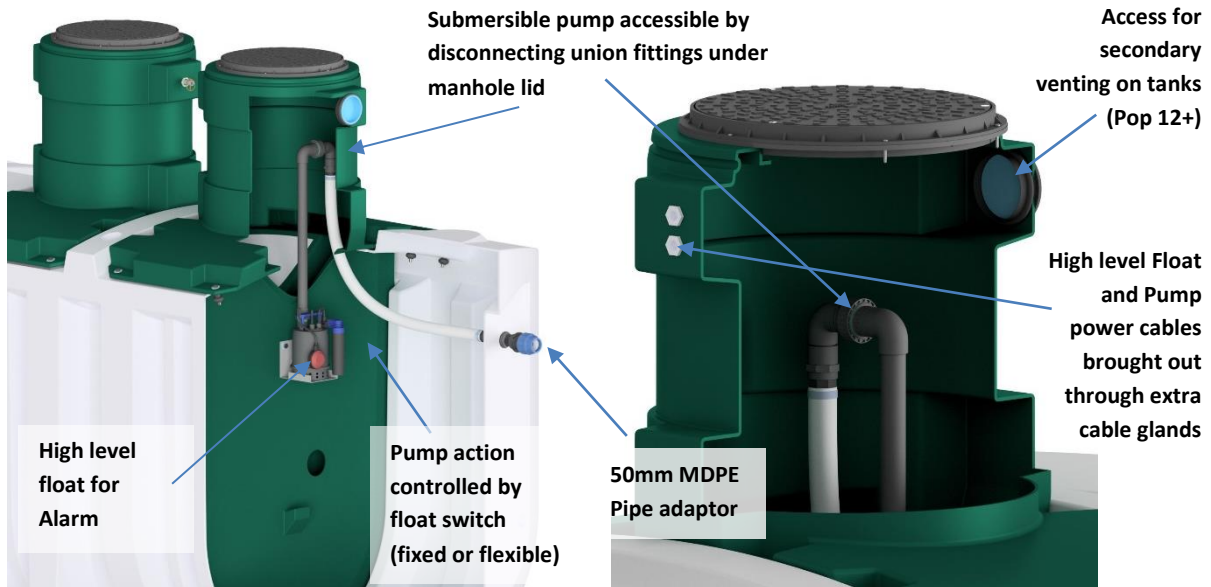
Figure 12: Tank Configuration in Pumped Outlet version
