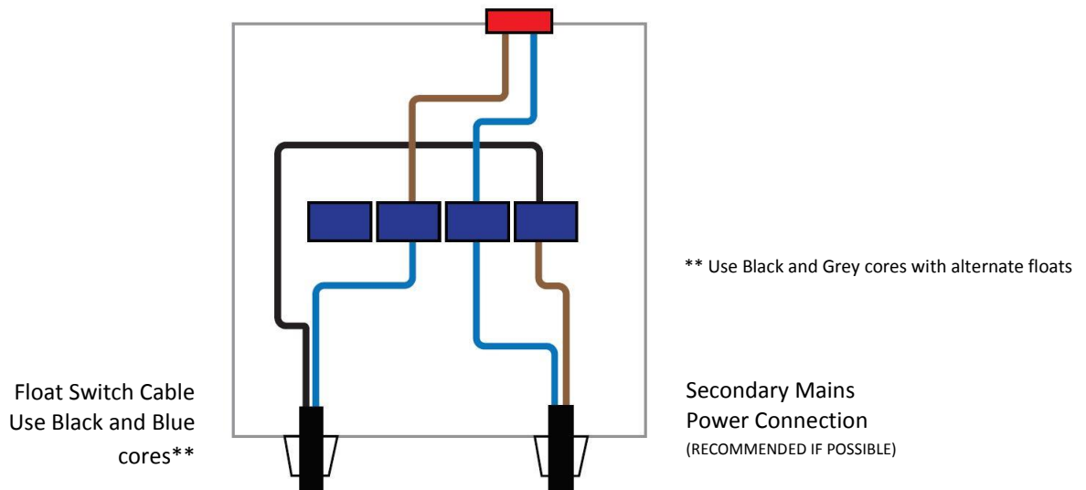
Figure 15: Wiring Connections inside Alarm box (Pumped Outlet Version)
