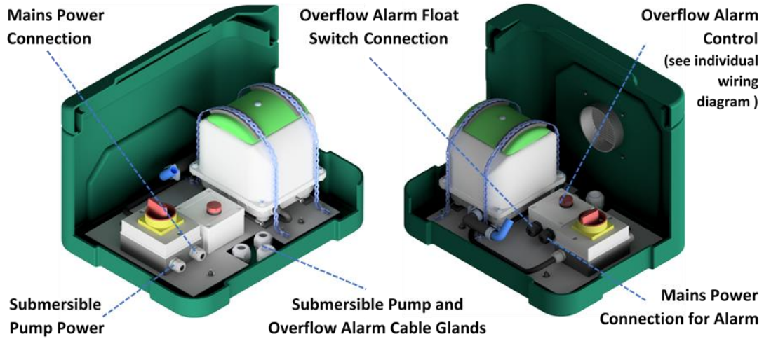
Figure 13: External Blower box assembly (Pumped Outlet version)
