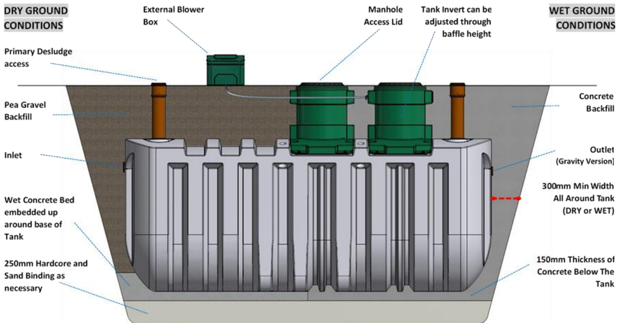
Figure 9: Typical Installation – Dry and Wet Ground Conditions
