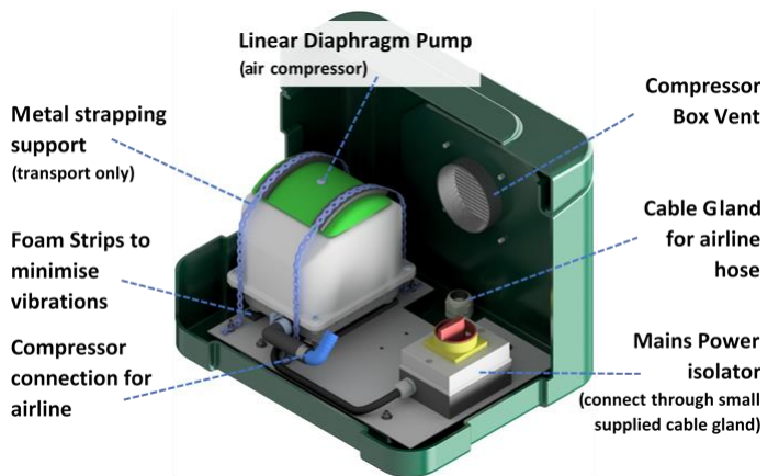
Figure 10: Inside the External Air Blower Housing
