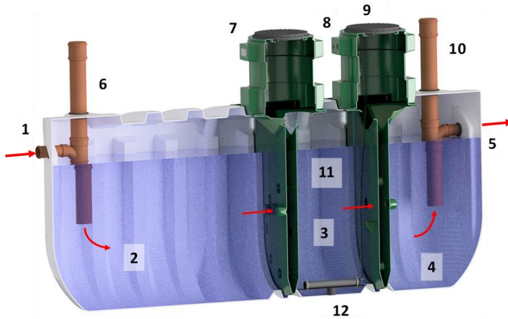
Figure 17: Process Description - HydroClear 12. (Air Blower & Electrics housed externally)
