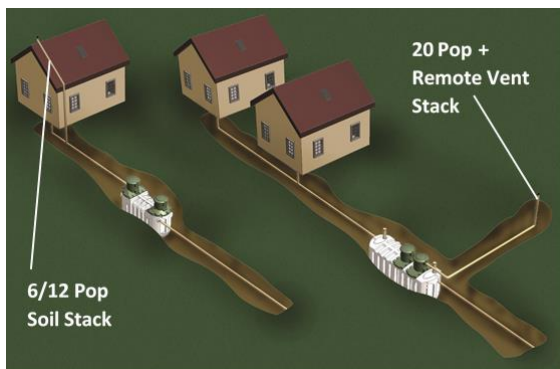
Figure 16: Ventilation
