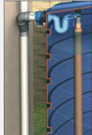
Inserting the filter unit onto the top of the pipe.
