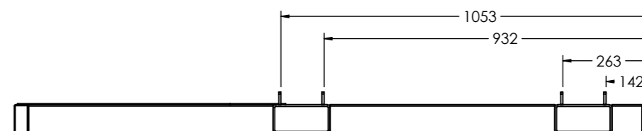
RIGHT VIEW
