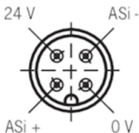
Figure 4 – Electrical connections
