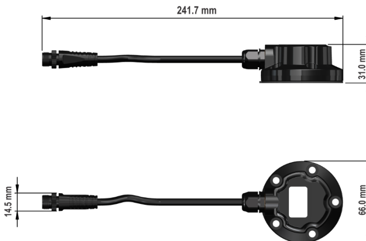
Figure 2 – TL400-I dimensions
