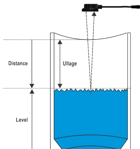
Figure 1 – TL400-I installation
