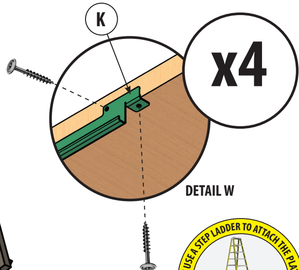
USA MADE ELEVATOR STAIR PLATFORM CONNECTION TO SUMMIT OUTDOORS ELEVATOR BRACKET SYSTEM PLATFORM (SOLD SEPARATELY)
