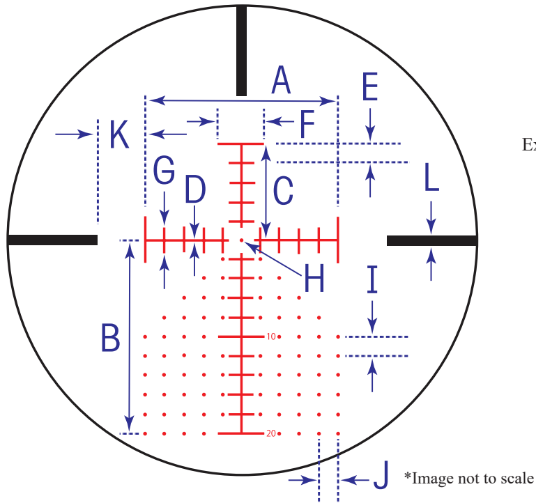
Illuminated MOA-H
