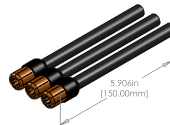
150.0MM EXIT LEAD EXTENSIONS (10 AWG) \varnothing 6.5MM MALE BULLETS PRE-SOLDERED
