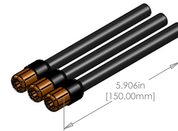
150.0MM EXIT LEAD EXTENSIONS (13 AWG) \phi 6.5MM MALE BULLETS PRE-SOLDERED
